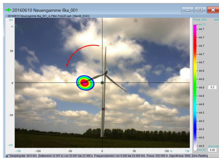
Figure 6: Acoustic picture of a wind turbine. As expected the maximum sound level is perceived from the blade at downward direction close to the blade tip
